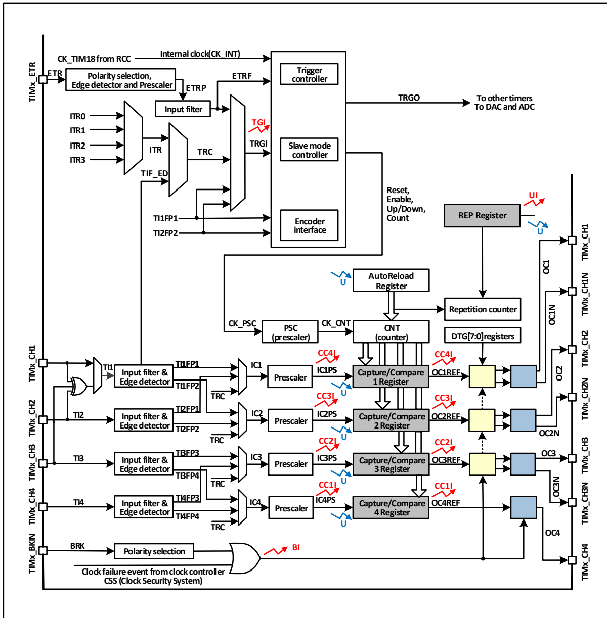
Figure 10-1 Block diagram of advanced-control timer structure
