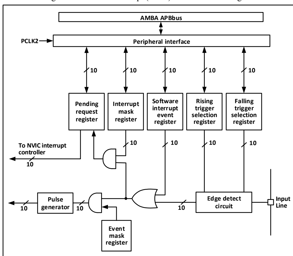
Figure 6-1 External interrupt (EXTI) interface block diagram
