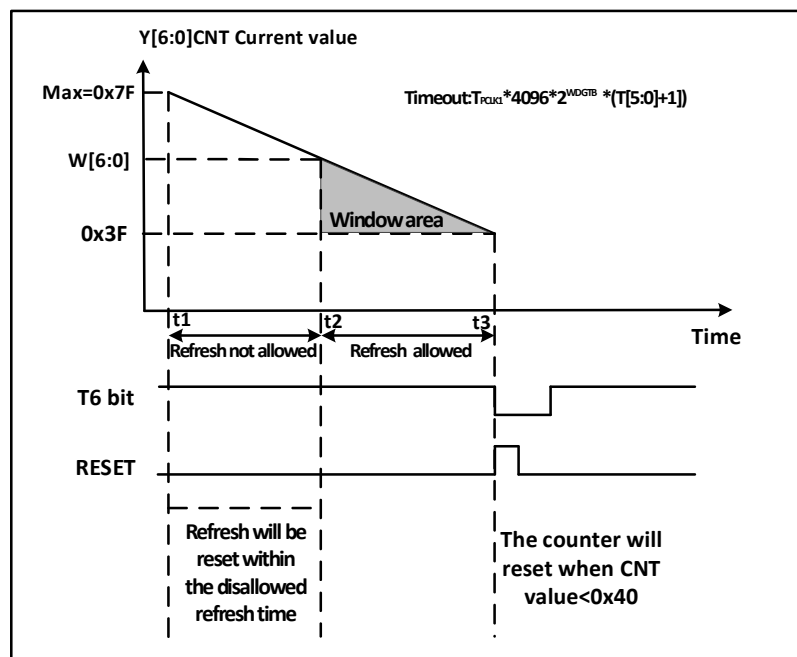
● Figure 5-2 Counting mode of Window Watchdog
